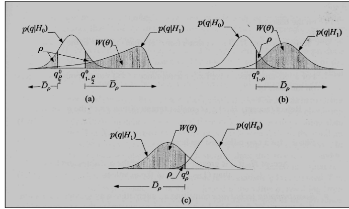
Figure 2. Confidence interval for (a) two-tailed index, (b) right-tailed index, (c) left-tailed index, where q_p^0 is the \rho proportion of q under hypothesis H_0 . [28]
