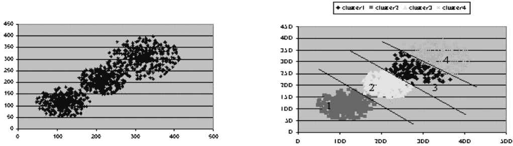
Figure 1. (a) A data set that consists of 3 three clusters, (b) The results from the application of K-means when we ask four clusters
