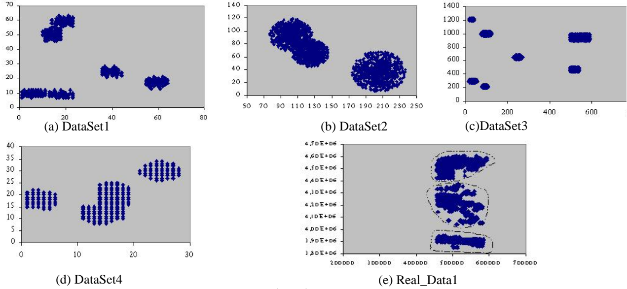
Figure 3 Datasets
